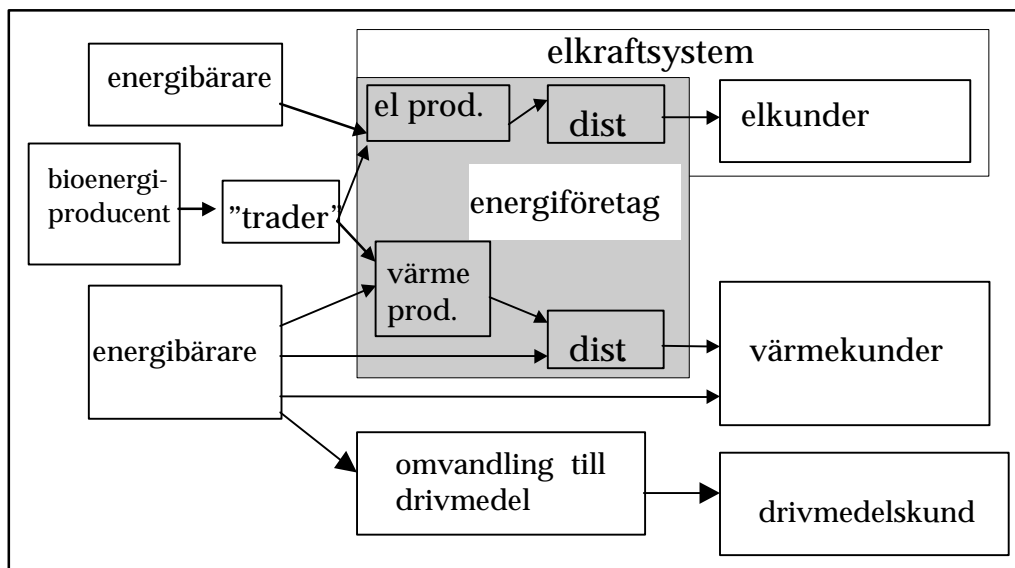
Figur 2 Energisystemet.
